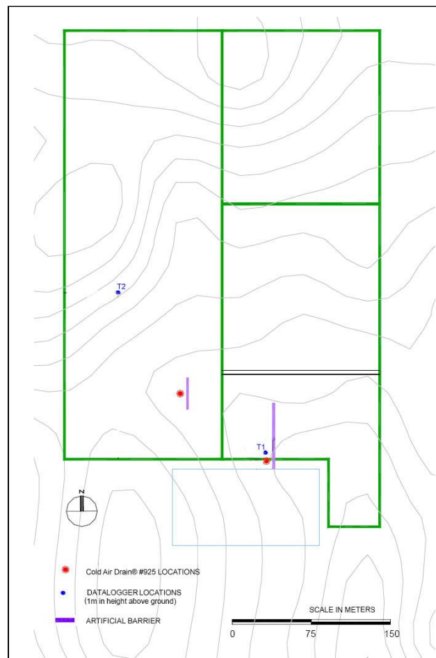
Figure 4: Datalogger, Artificial Barrier, and Cold Air Drain ® Locations
